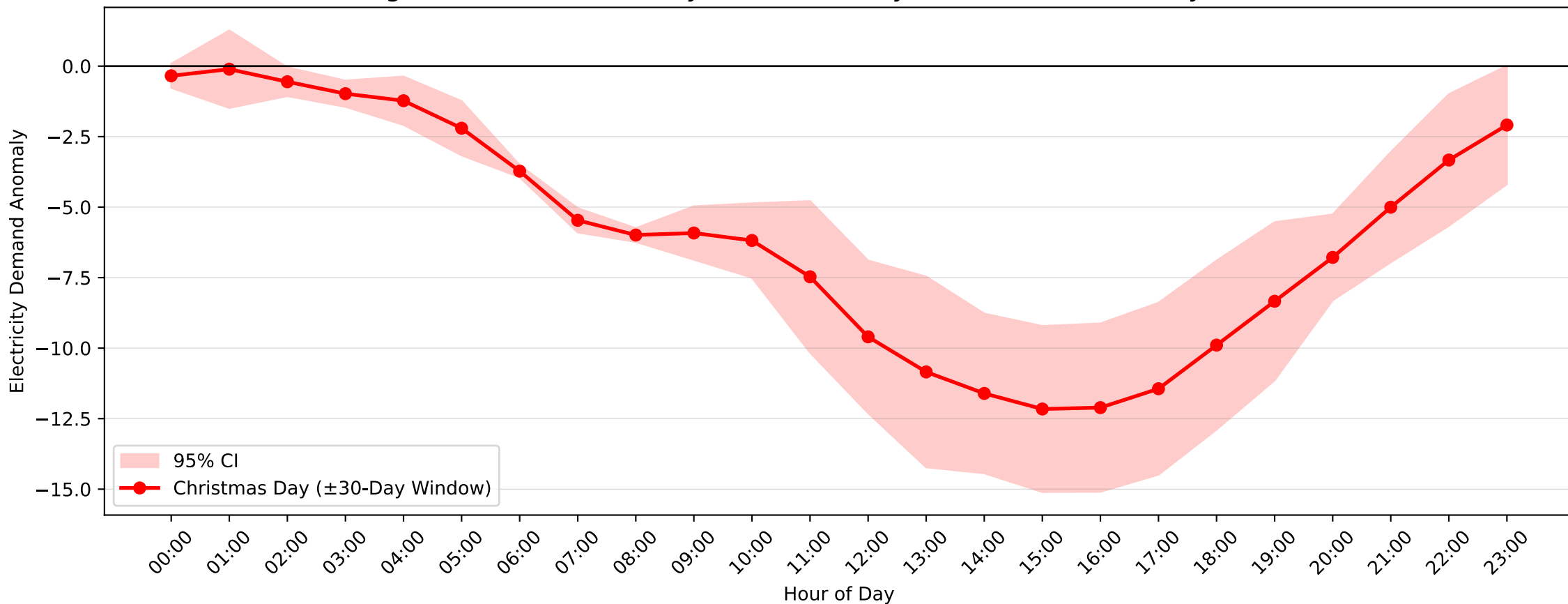
Kogarah Demand Anomaly: Christmas Day (2015-2016, \pm 30 -Day Window)
